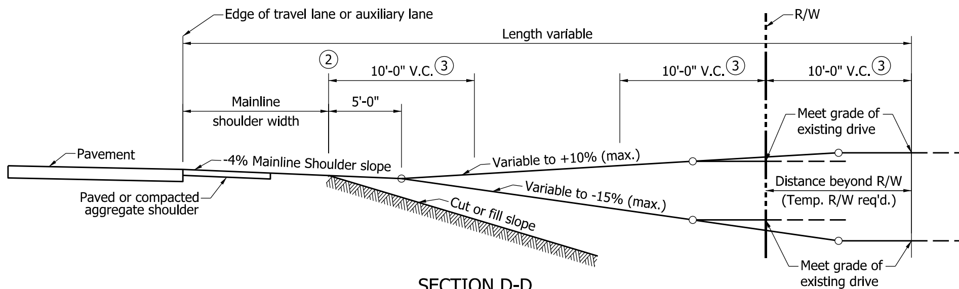
SECTION F-F (APPROACH GRADE FOR CUT OR FILL TO BE USED WITH PAVED SHOULDER 8'-0" OR WIDER)
