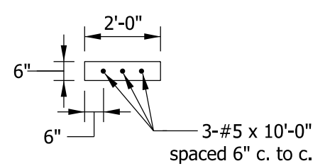
TYPICAL CORNER REINFORCING FOR CLASS II DRIVE
