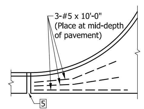
CONCRETE CURB AND GUTTER
